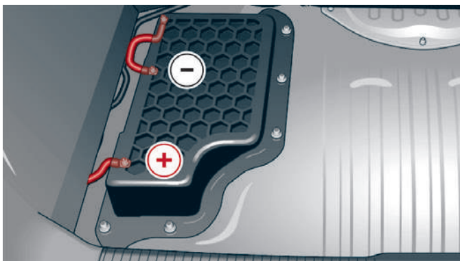
Disconnecting the battery
