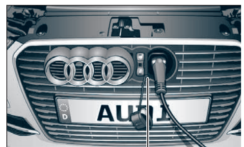
Front charging socket
